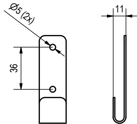
Bracket Detail
