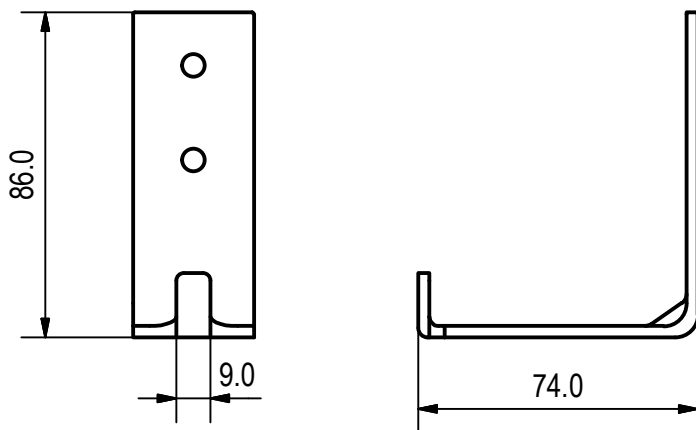
Bracket Detail
