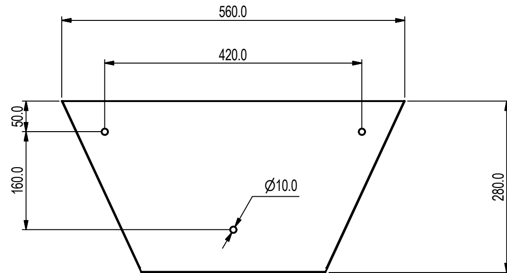
Back View
