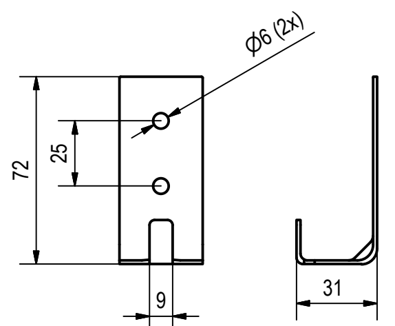
Bracket Detail
