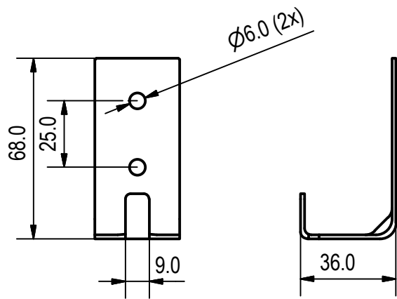
Bracket Detail
